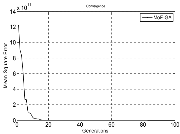
Fig. 7. Mean square error versus generation for h=25m.
