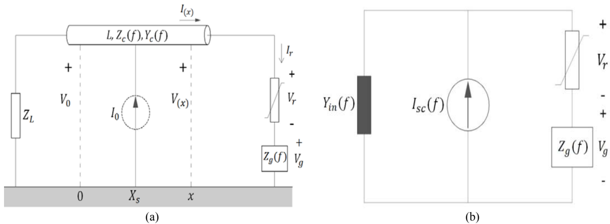
Fig. 2. (a): Frequency-domain representation of figure 1 in which the overhead line and grounding system are represented by transmission line and linear impedance respectively and surge current by current source I_0(t) , (b): Norton equivalent circuit viewed across arrester.
