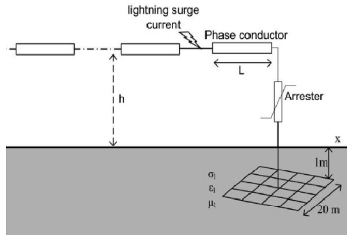
Fig. 1 Overhead line connected to grounded arrester and subjected by direct lightning strike in which grounding system is represented by grid grounding [8].
