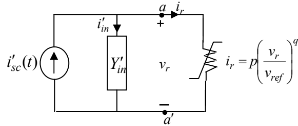
Fig 4. Simplified equivalent circuit of the figure 3.
