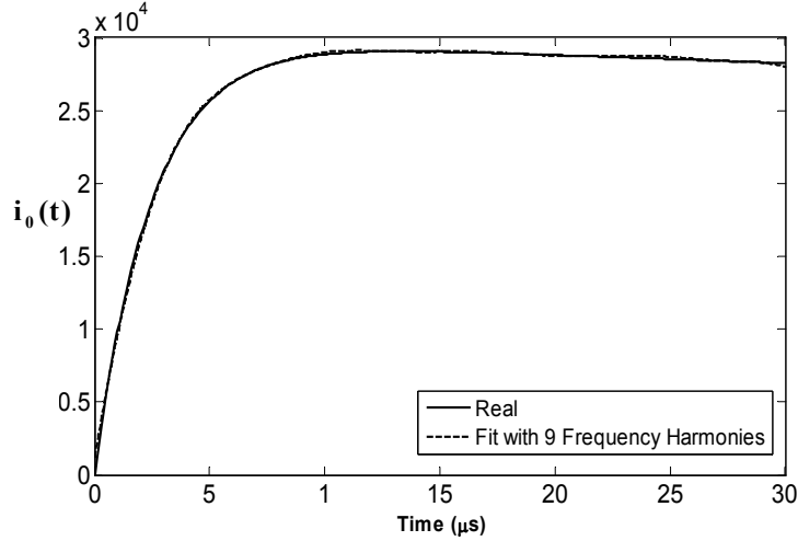
Fig. 3. Approximating the current source I_0(t) by nine frequency harmonies.
