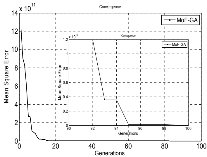
Fig. 6. Mean square error versus generation for h=10m.
