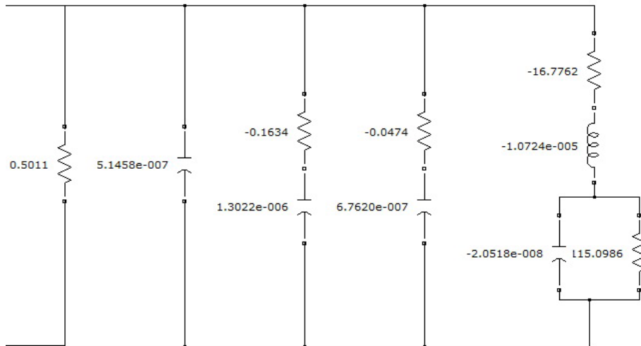
Fig. 8. Equivalent circuit of grid grounding system by VF for conductivity=0.01S/m. Resistors, inductors and capacitances are in \Omega , H and F respectively.
