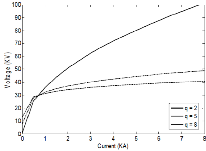
Fig. 5. i-v characteristic of the arrester.
