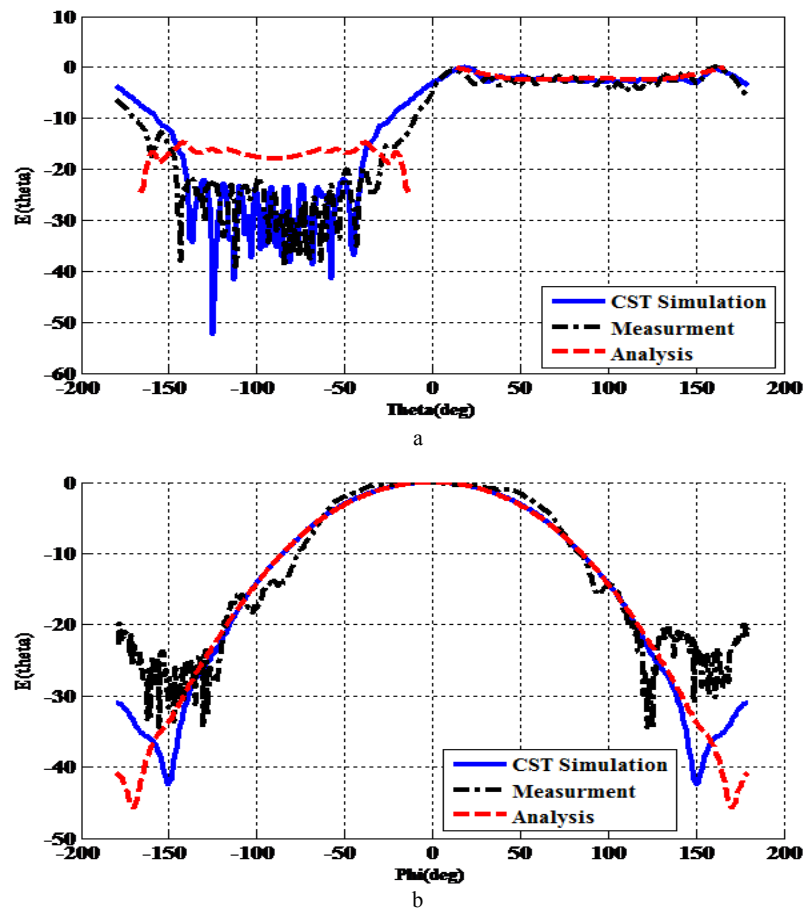
Fig. 8 .The Radiation Pattern of the Realized Antenna. (a) \phi=0^\circ plane, (b) \phi=90^\circ plane
