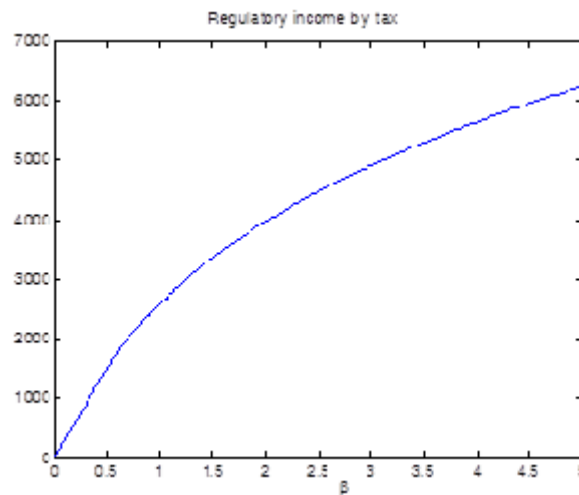
Fig.13. The impact of freedom parameter ( \beta ) on the regulatory income.
