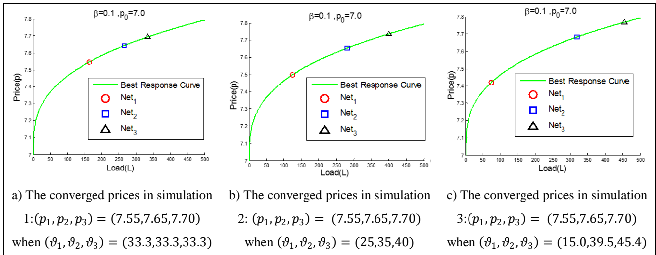
Fig.11.The converged prices in simulations
