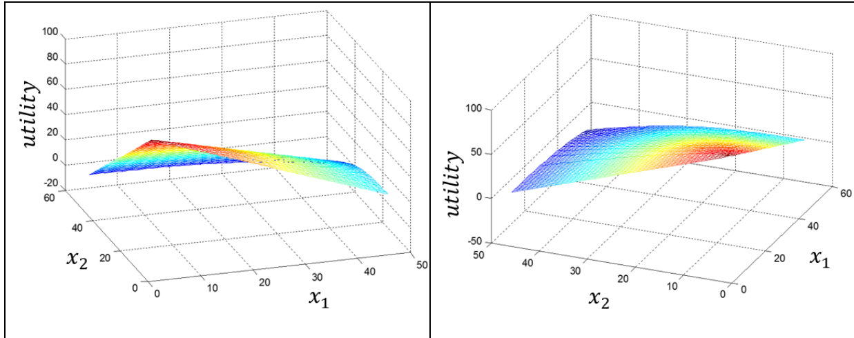
Fig.4. The concave surface of utility function for a client with H^i = 90, w^i = (1,1), \theta = (1,1), p = (7,9)
