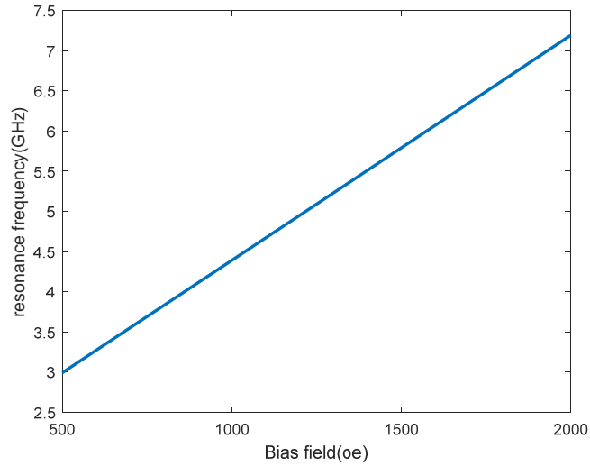
Fig. 7. Resonance Frequency of ferrite rods.
