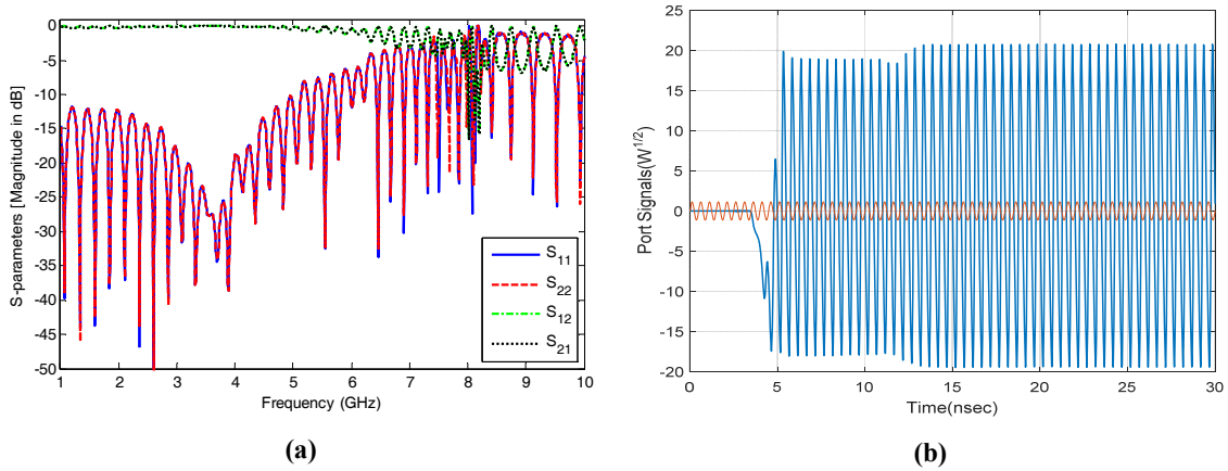
Fig. 3. (a) Scattering parameters of reference TWT (b) Input &amp; output signals.
