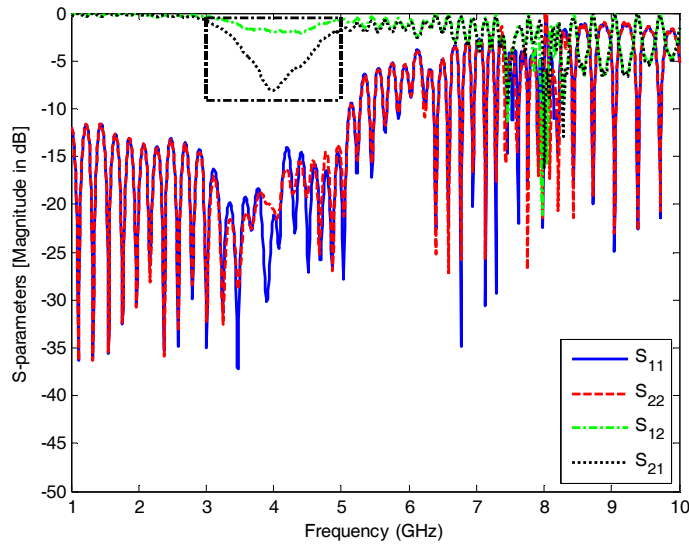
Fig. 8. Scattering Parameters of new structure for reducing 2 nd harmonic
