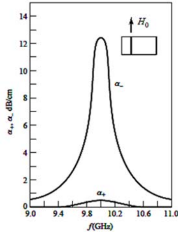
Fig. 1. Frequency response of rectangular waveguide isolator.
