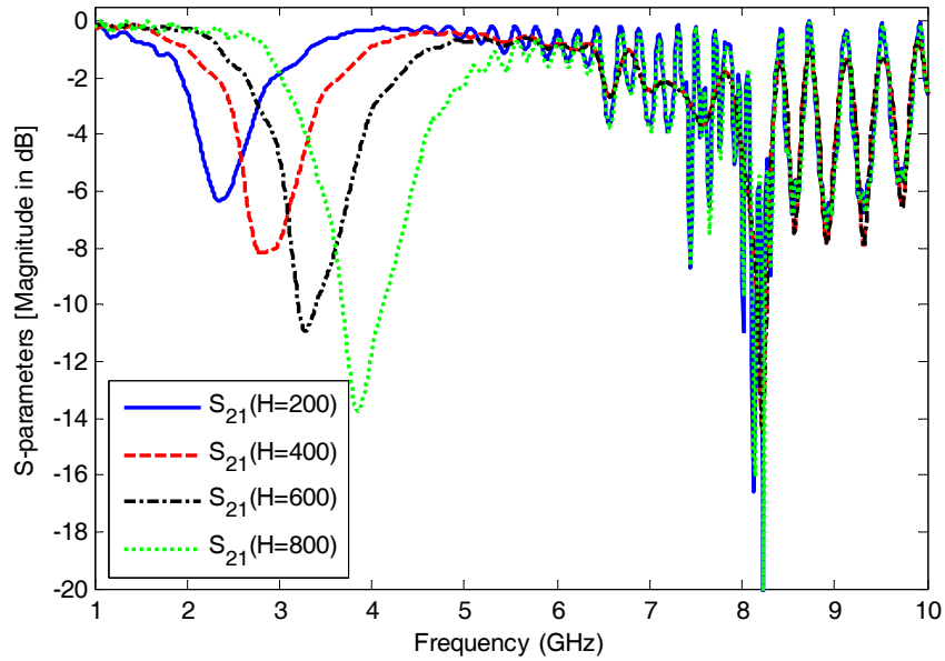
Fig. 6. Center Frequency of Band Stop Filter Based on Different Bias Field
