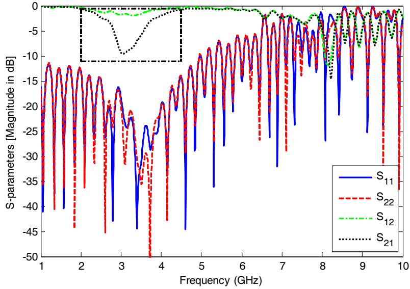
Fig. 5. Non-Reciprocal Scattering Parameters of Ferrite Loaded SWS
