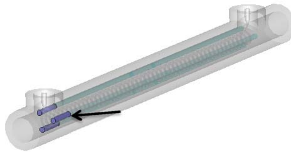
Fig. 4. New SWS created by removing a portion of dielectric rod and replacing by ferrite rods.
