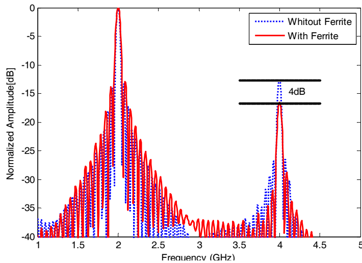
Fig. 9. Output signals spectrum for both structures show that 2 nd structure has lower harmonic
