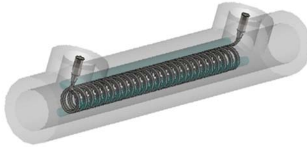
Fig. 2. Reference TWT operate in 2-5 GHz.
