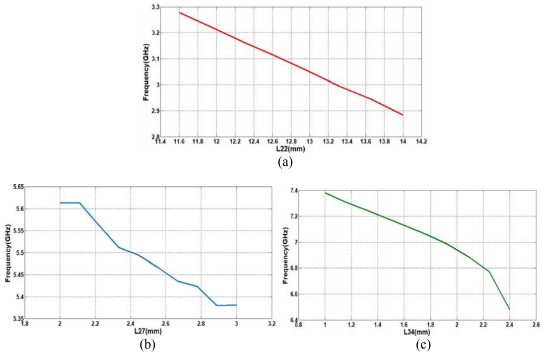
Fig. 3. The resonance frequency versus length, (a) the loop resonator length, (b) DMS length, and (c) the open stubs length.
