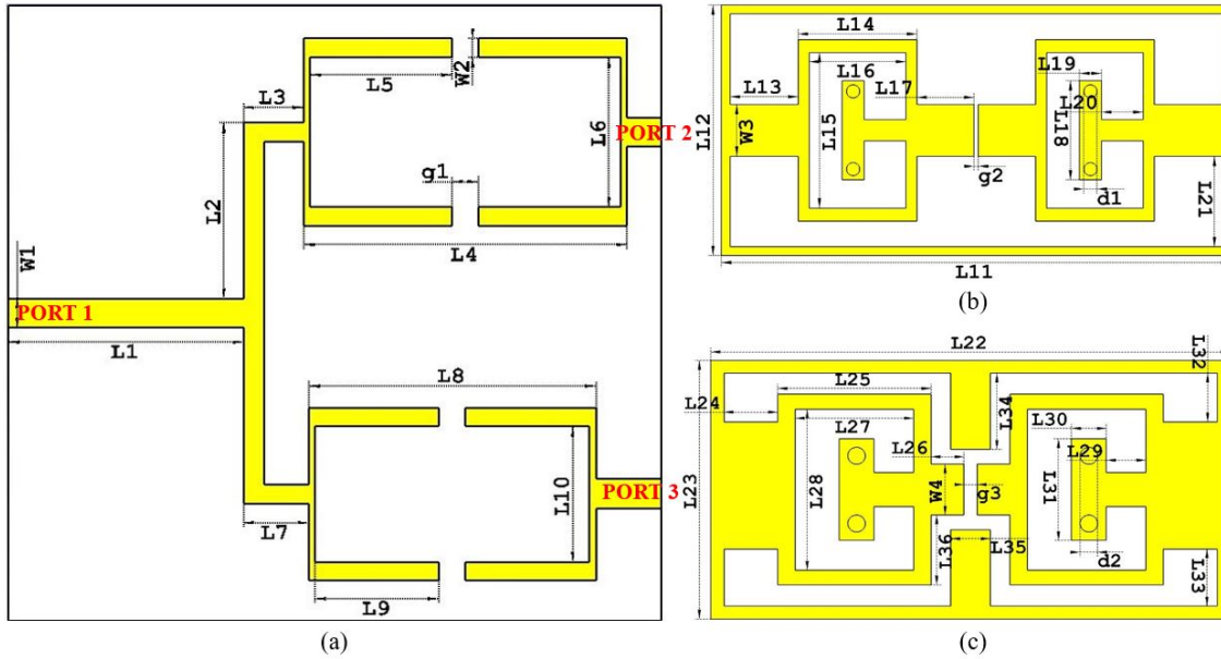
Fig. 1. Structure of proposed multi-channel diplexer. (a) General configuration of two channel diplexer with bandpass filter unit cell, (b) quad-channel diplexer with dual-band unit cell, (c) six-channel diplexer with tri-band unit cell.
