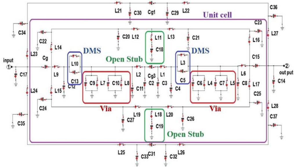
Fig. 2. LC circuit of the filter.
