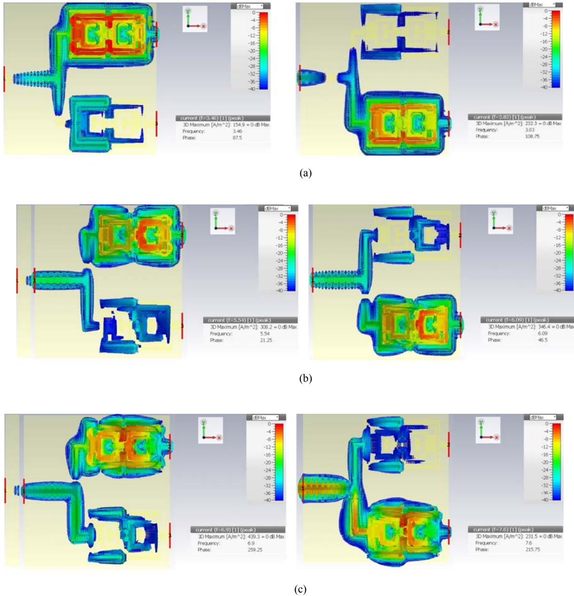
Fig. 6. Surface current distribution in six-channel diplexer at different frequencies. At (a) 3.4 and 3.8 GHz, (b) 5.5 and 6.1 GHz, and (c) 6.9 and 7.6 GHz.
