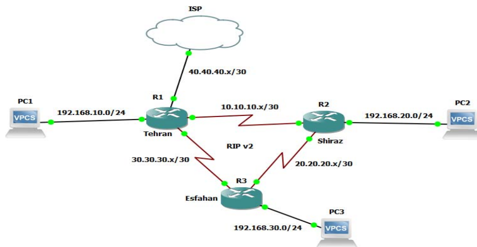
Fig. 3. RIPv2 application scenario
