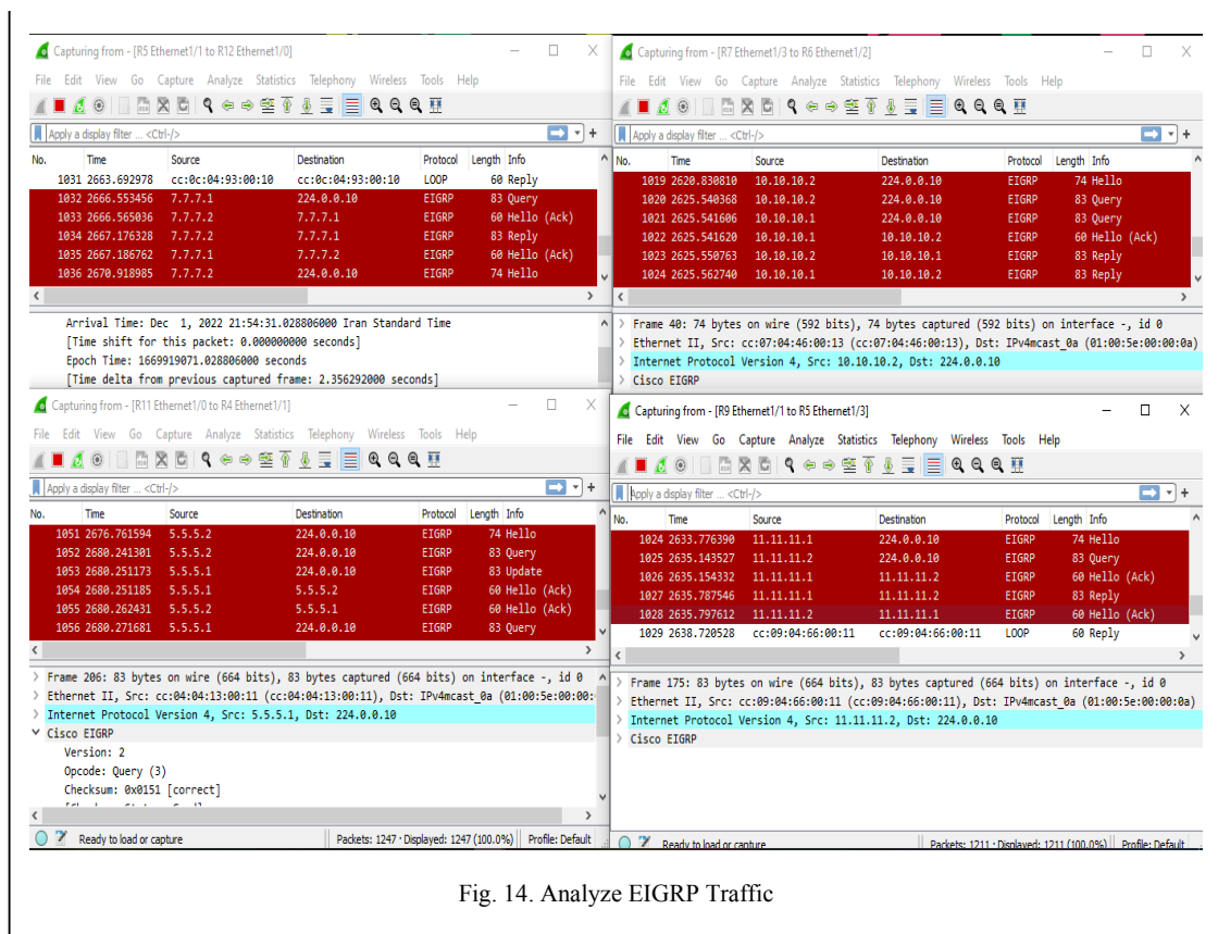
Fig. 14. Analyze EIGRP Traffic
