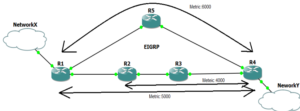
Fig. 7. EIGRP terminology
