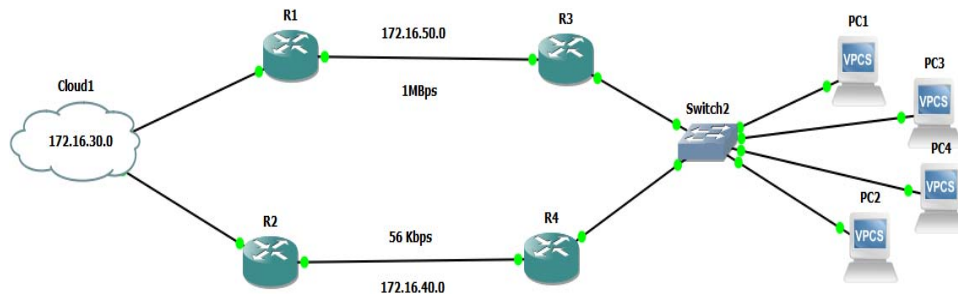
Fig. 2. RIPv2 load balancing
