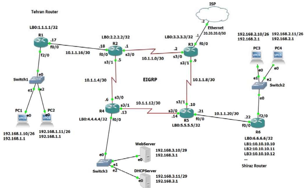
Fig. 9. EIGRP Scenario in GNS3
