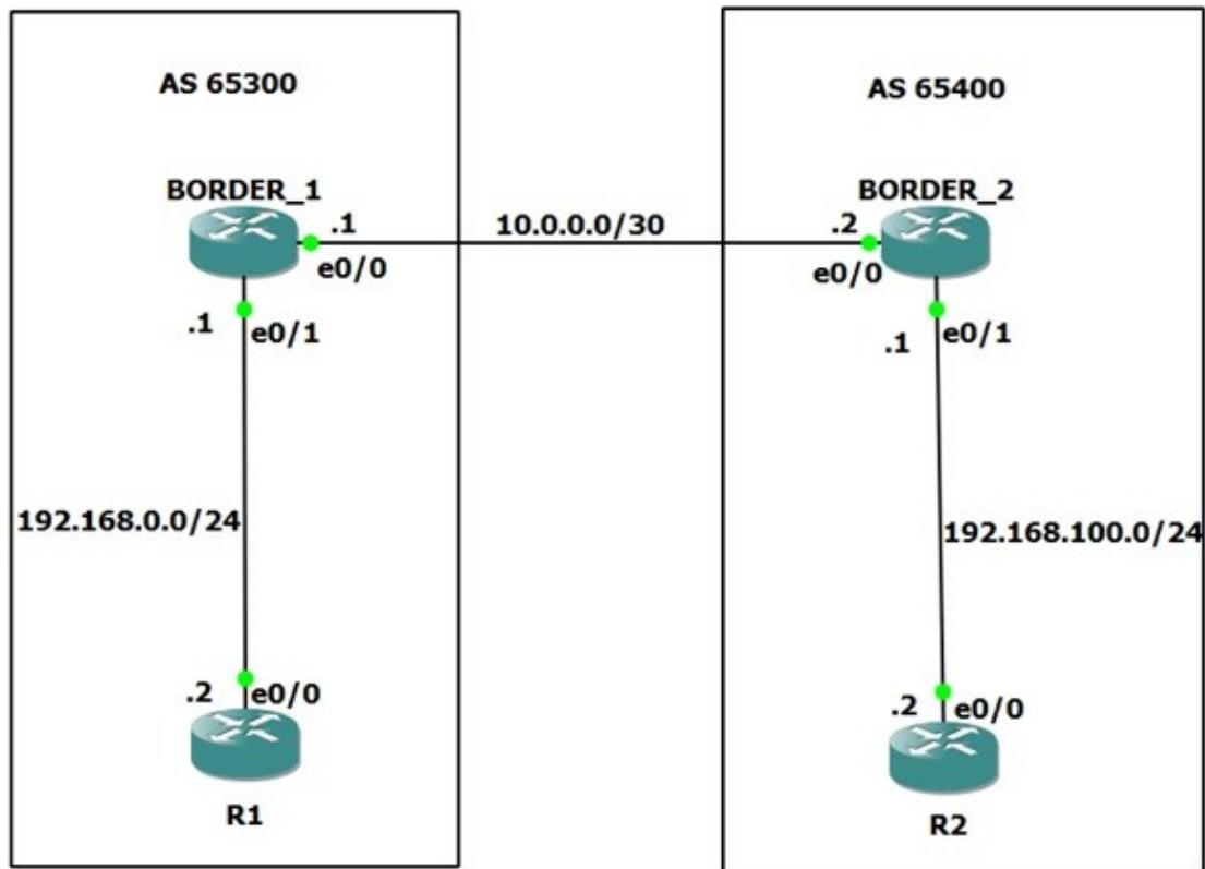
Fig. 6. BGP Scenario in GNS3
