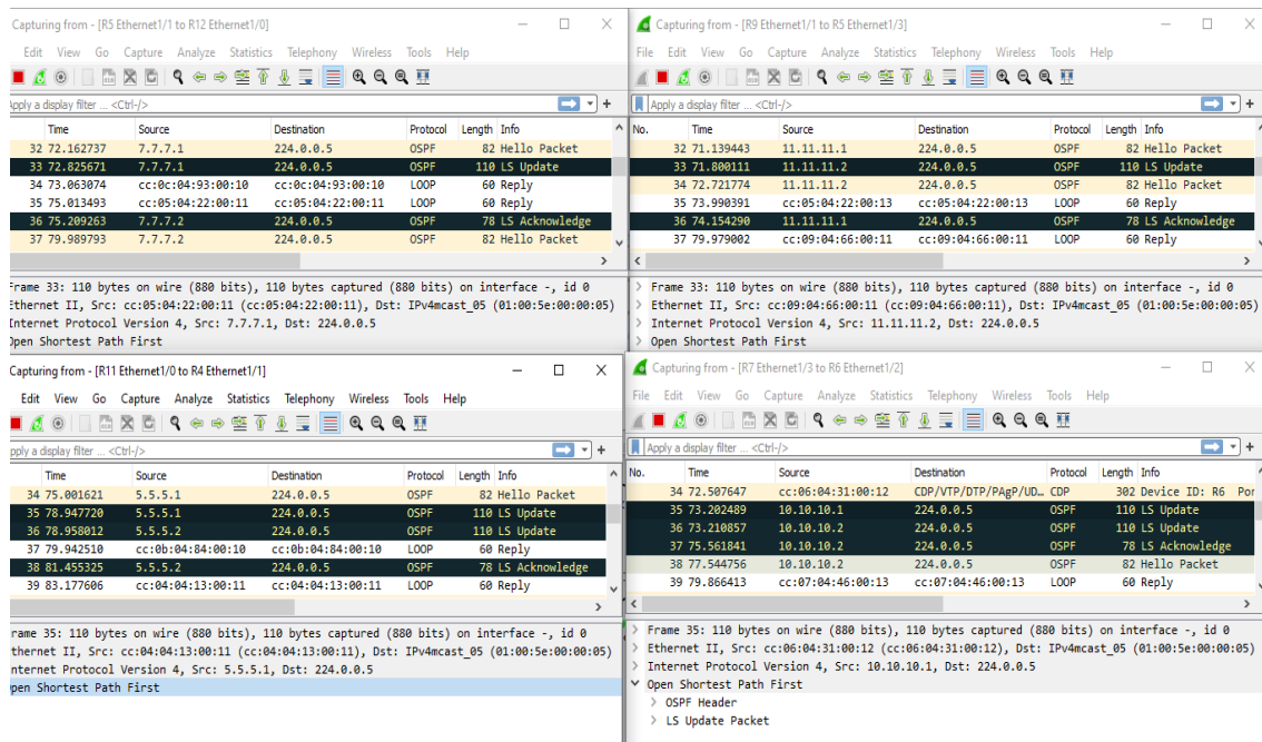
Fig. 15. Analyze OSPF Traffic
