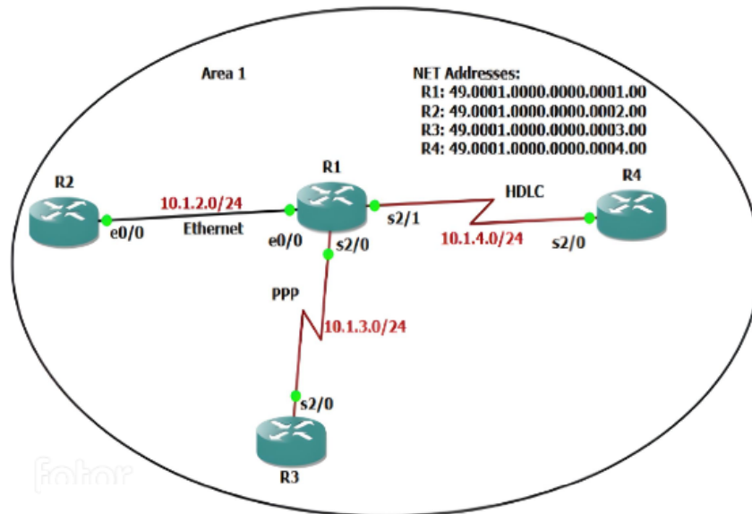
Fig. 10. ISIS Scenario in GNS3
